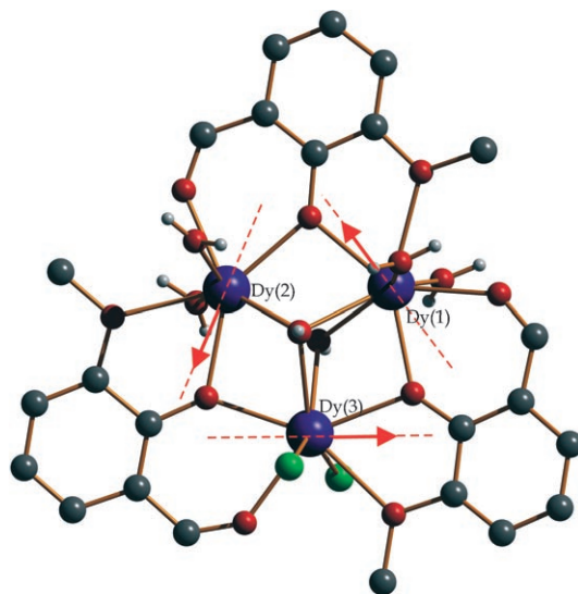
Figure 1. Structure of the triangular units in 1 and 2 . [19] The structure with two chloride ions coordinated to \text{Dy}(3) was used in the ab initio calculations. Color scheme: blue \text{Dy}^{\text{III}} ; red O; green Cl; dark grey C; white H. The dashed lines show the calculated anisotropy axes on the dysprosium fragments and the arrows show the ordering of local magnetizations in the ground state of the complex.
