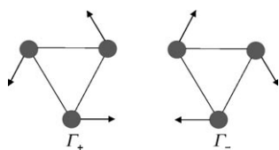
Scheme 1. The two components of the ground Kramers doublet in 1 and 2 . The arrows show the direction of magnetization on the dysprosium sites.
